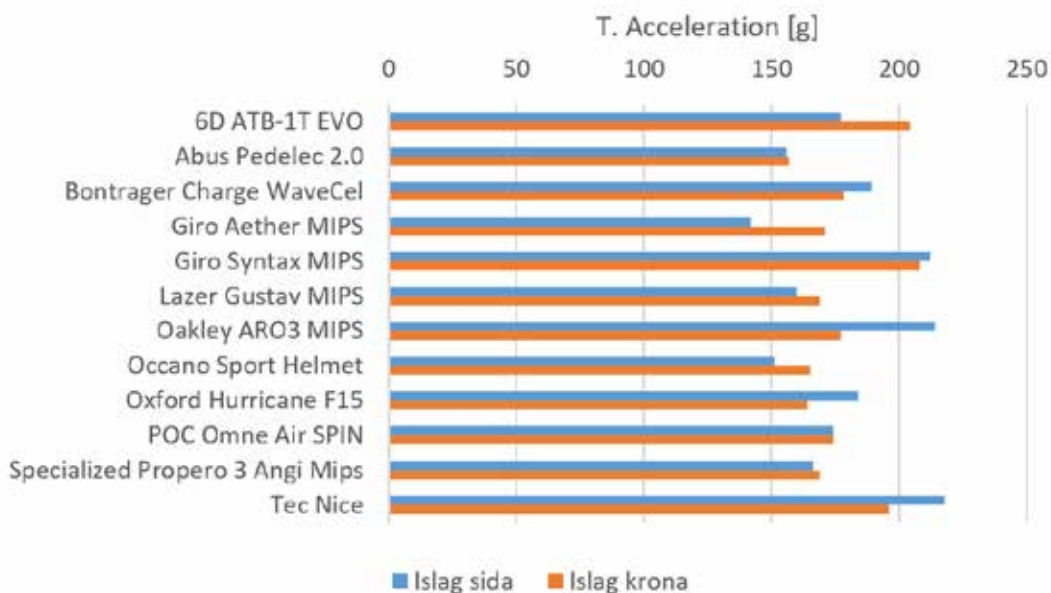
Figure 1. Shock Absorption measuring linear acceleration
